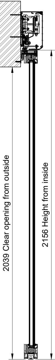
3. SECTION - NTS
