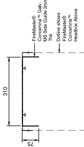
END SECTION SIDE GUIDE DETAIL
