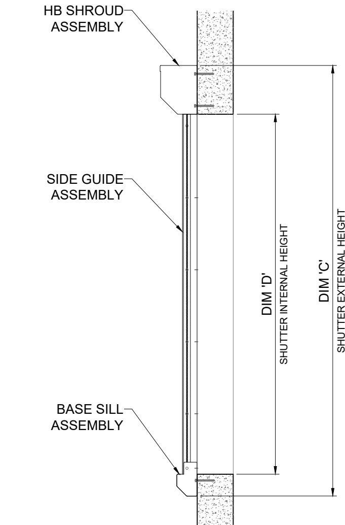
3 SECTION
