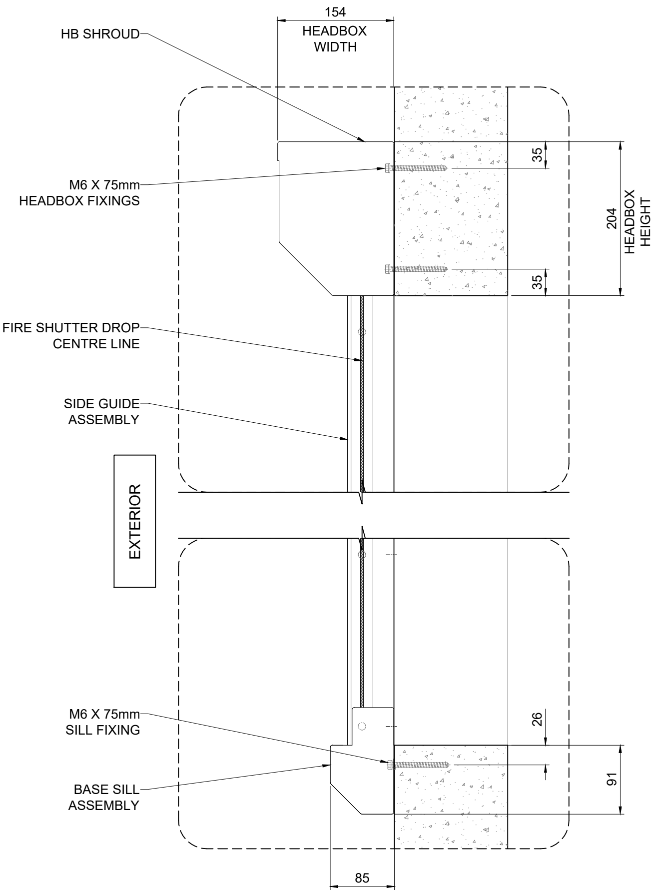
2 SECTION DETAILS
